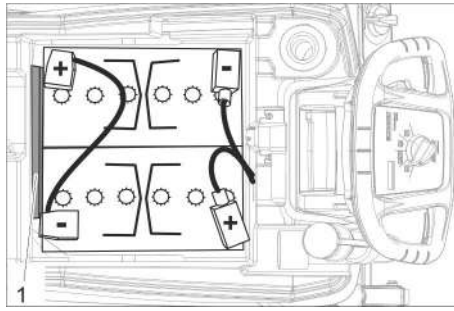
Akku 6.654-290,0
